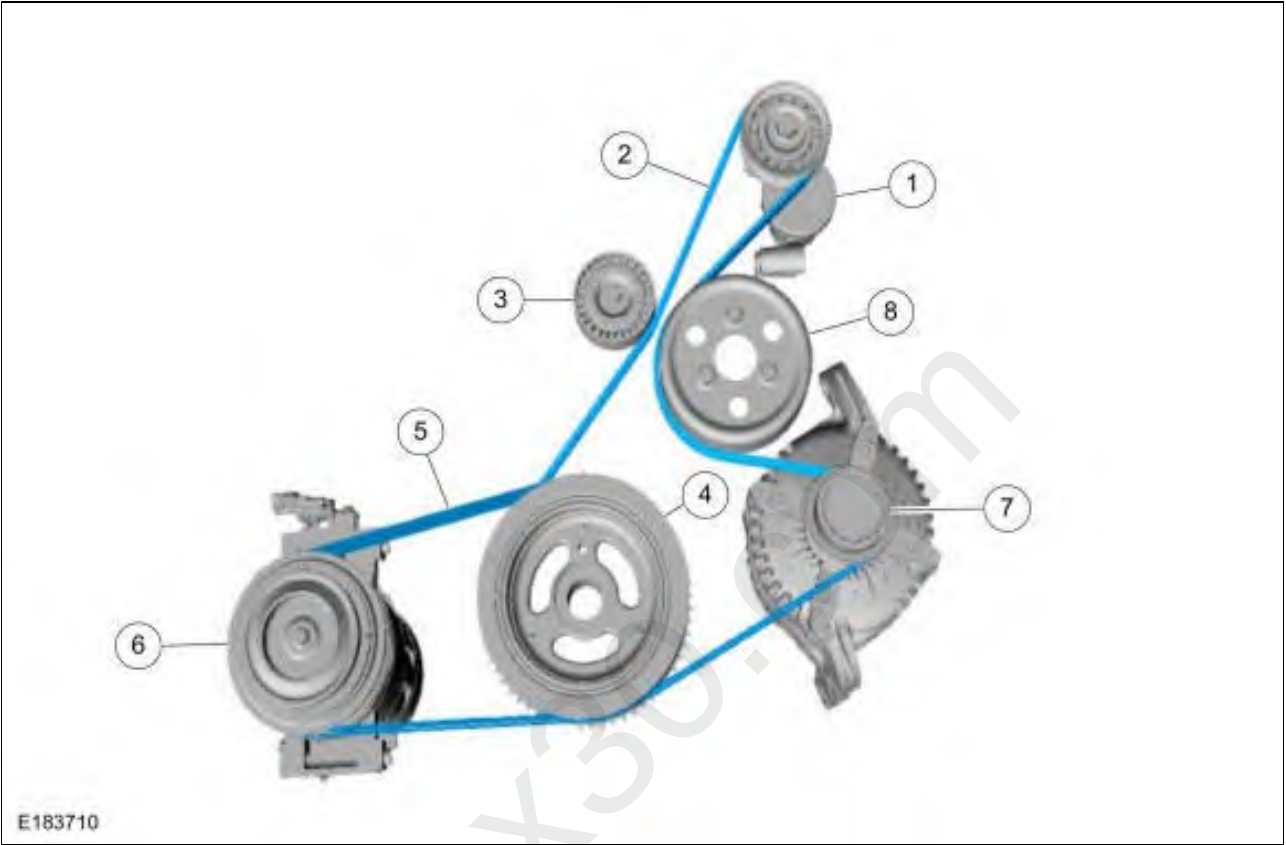
Fig 1: View Of Drive Belt Routing And Pulley
